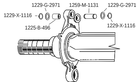
STD. ANCHOR PIN HARDWARE
