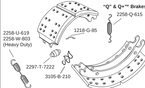
"Q" & Q+™ Brakes
