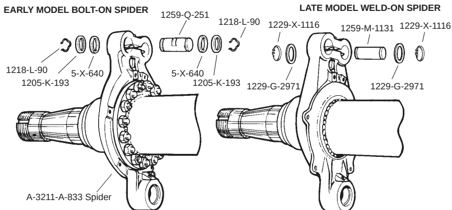
EARLY MODEL BOLT-ON SPIDER
