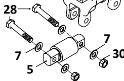
Bar Pin Style Axle Connection
