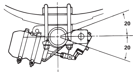
Brake Clocking
