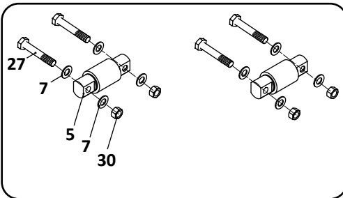
Axle, Bar Pin Style Connection Kit
