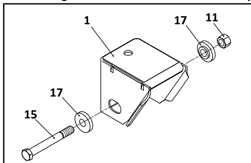
Welded Alignment Pivot Connection Assembly
